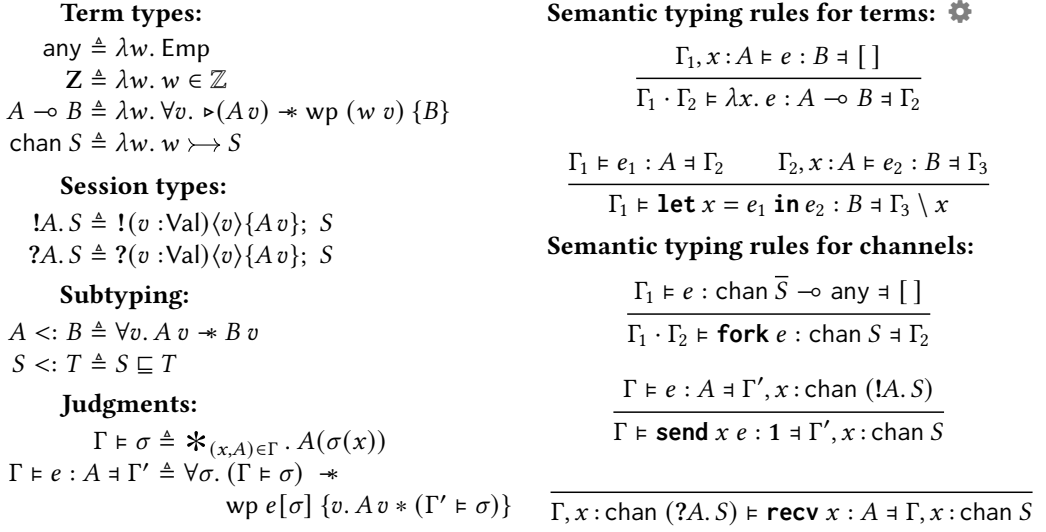
Fig. 7. Typing judgements and type formers of the semantic type system.
